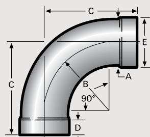
90° Short Radius Elbow
