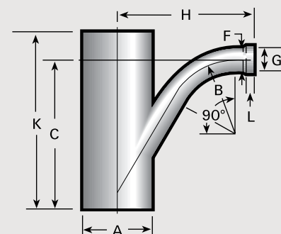
90° TY (one end expanded)
