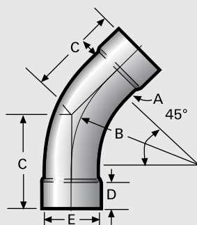
45° Standard Radius Elbow
