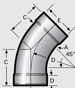
45° Short Radius Elbow
