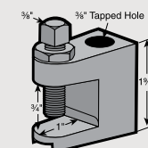
Beam Clamp
