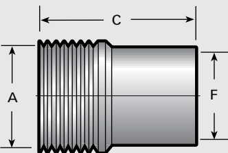
Male Adapter
