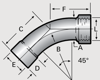
45° Female Adapter Elbow
